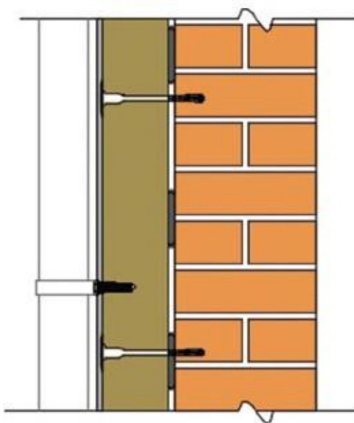
Detail 28 - Lightweight items such as rain water pipes, lightweight signs etc
