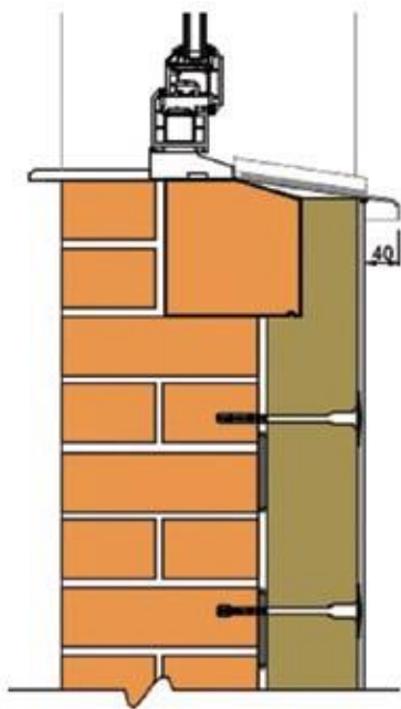
Detail 7 - Existing feature sills with existing retained windows
