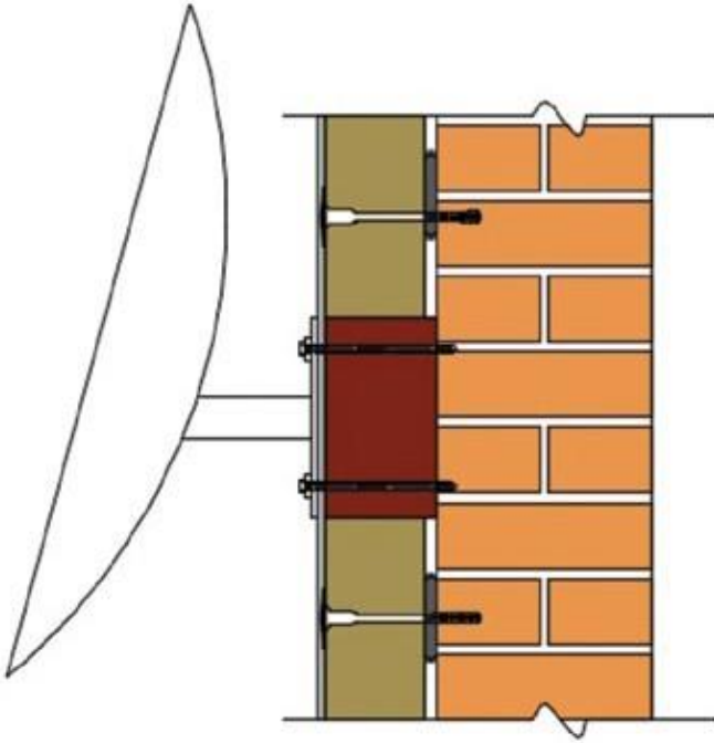
Detail 27 - Heavy items such as satellite dishes, aerials, washing lines etc
