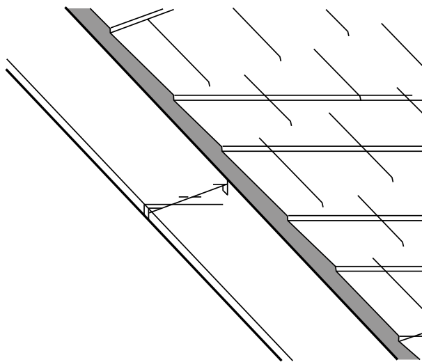
Detail 59 - 3D image on verge or fascia trim connection profile
