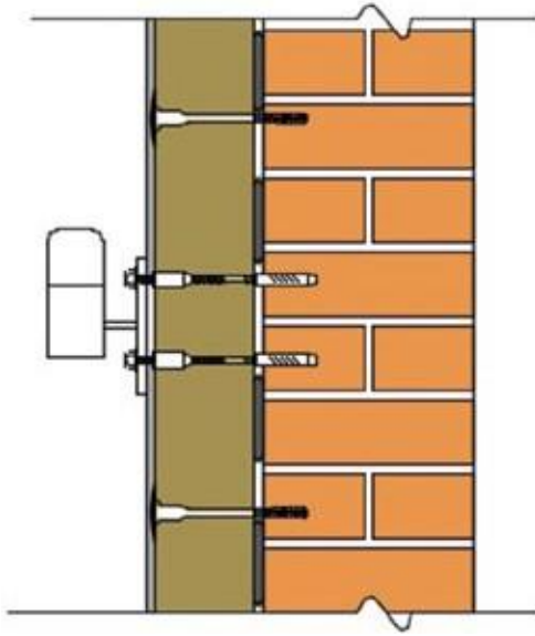
Detail 29 - For post fix items such as lights, satellite dishes, aerials etc
