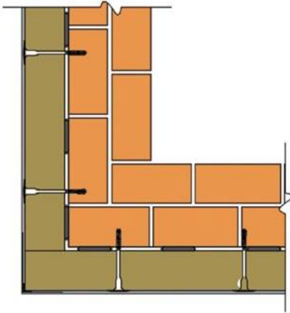
Detail 49 - Typical external corner
