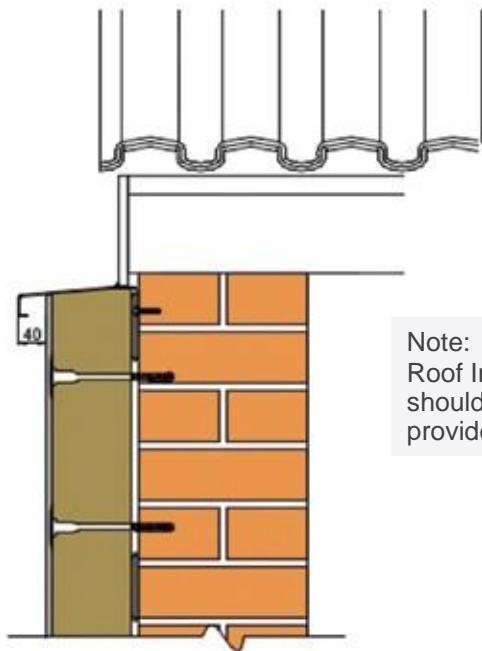
Detail 24 - Detail at flush verge
