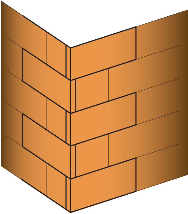
Detail 52 - 3D image on external corner when boarding
