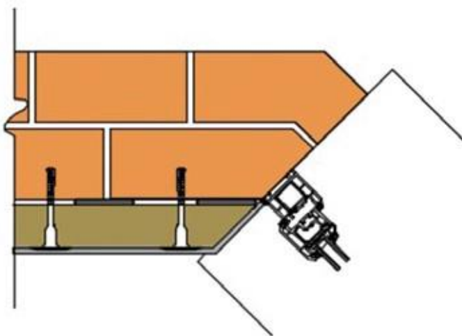
Detail 18 - Detail where system meets an existing bay window
