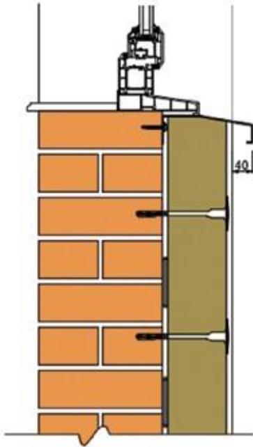
Detail 6 - Existing windows and sills with new under sill trim
