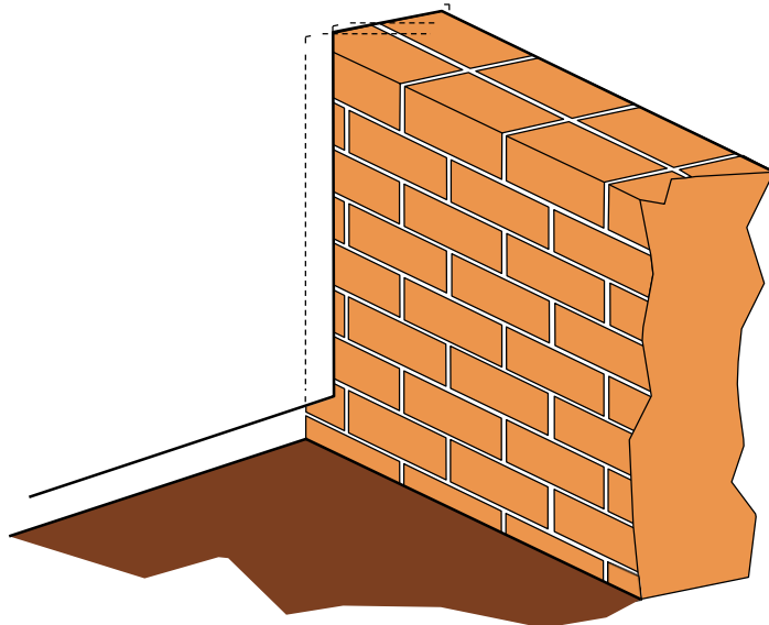
Detail 55 - 3d image of wall abutment
