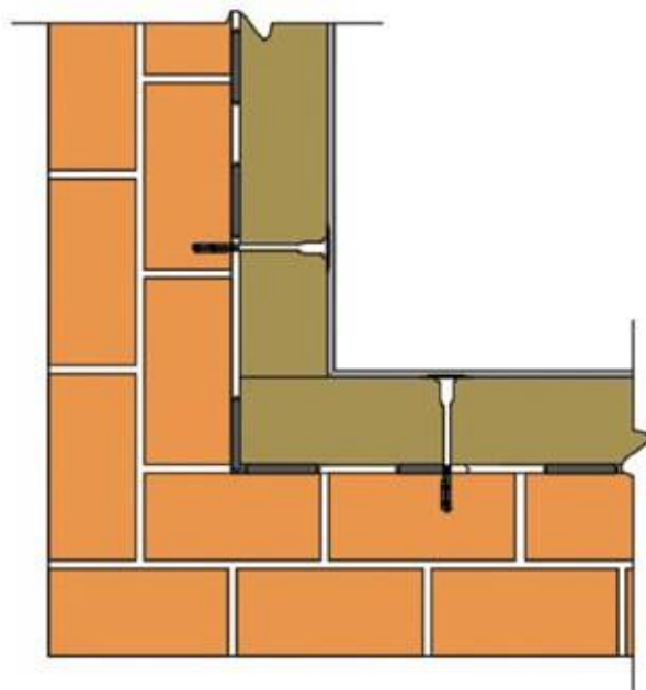
Detail 50 - Typical external corner
