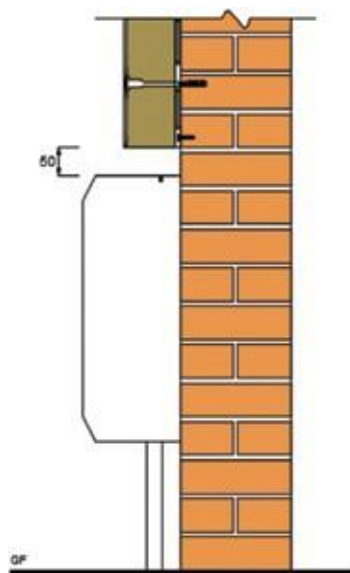
Detail 37 - Section through gas box
