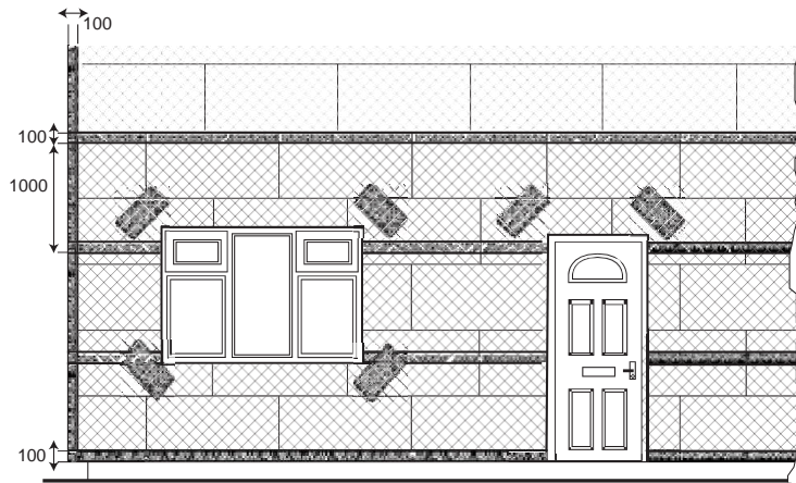
Detail 54 - Typical meshing and stress patches elevation
